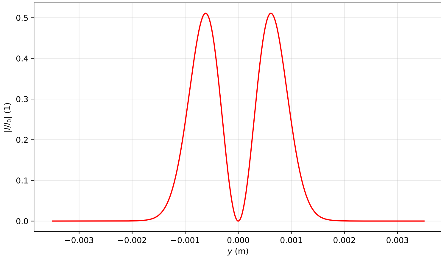
Intensity profile I(x=0, y, z=1.433)/I_0 , P_{in}=0.5P_{cr} , artificial time
